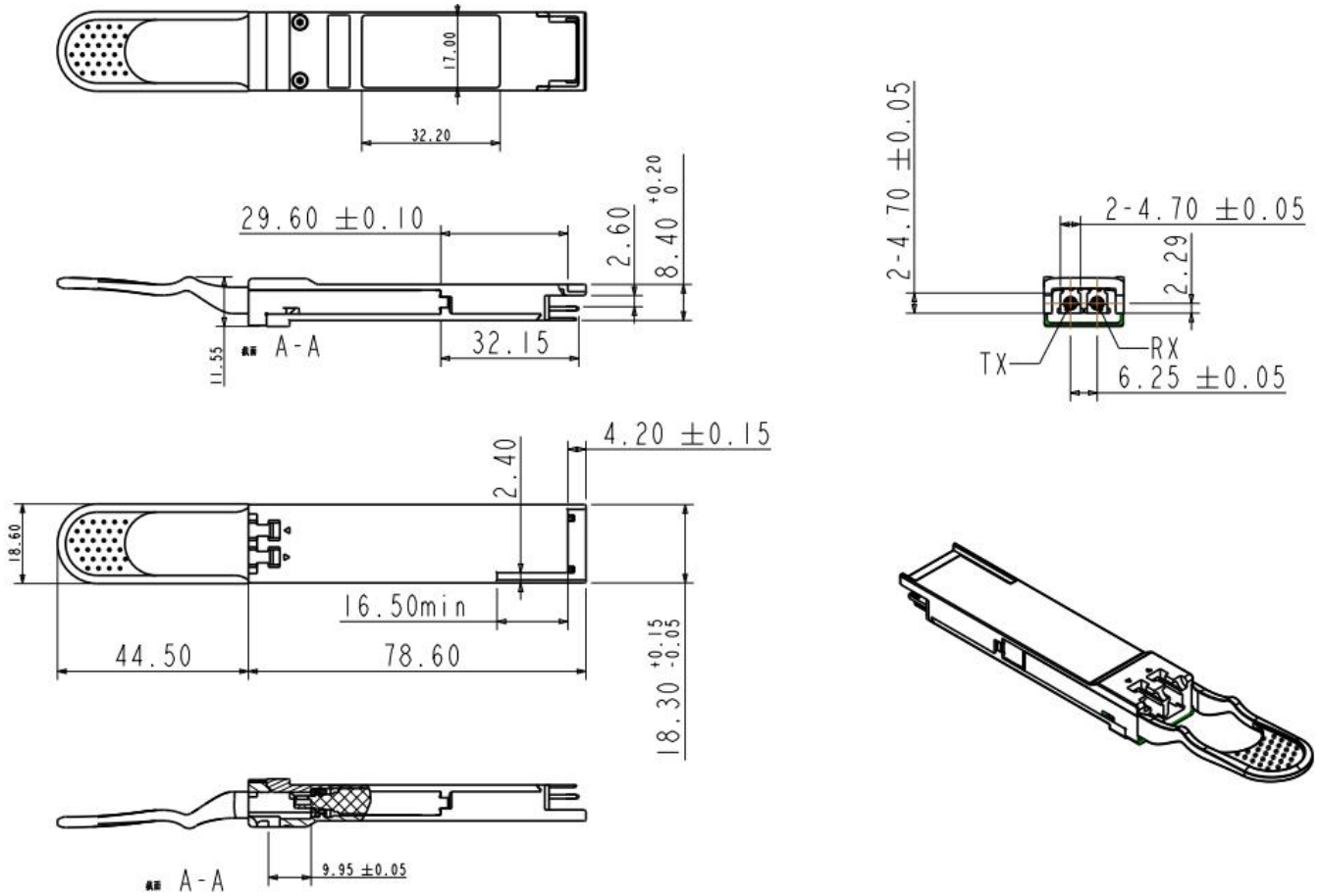
Figure 9 . Mechanical Specifications
